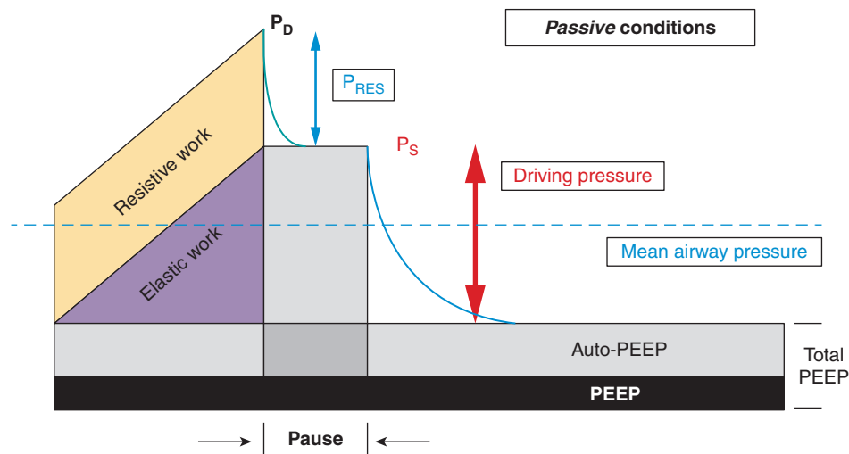
Fig. 53.9 Partitioning of inflation work under passive conditions of constant inspiratory flow. The horizontal axis is time. During constant flow, time is an analog of volume. Total positive end-expiratory pressure (PEEP) the sum of applied and auto-PEEP has an associated energy cost during inflation.
