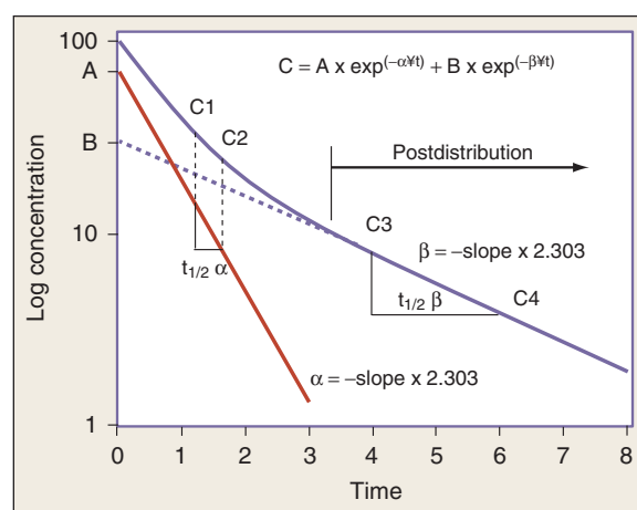
Fig. 139.4 Log concentration-time curve for a two-compartment model after intravenous administration, illustrating a distribution period ( \alpha ) and postdistribution period ( \beta ). Concentrations C_1 and C_2 reflect both distribution and elimination processes, whereas concentrations C_3 and C_4 reflect postdistribution elimination processes.
